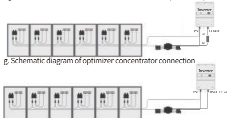
g. Schematic diagram of optimizer concentrator connection h. Use the RSD port of inverter to supply the concentrator
