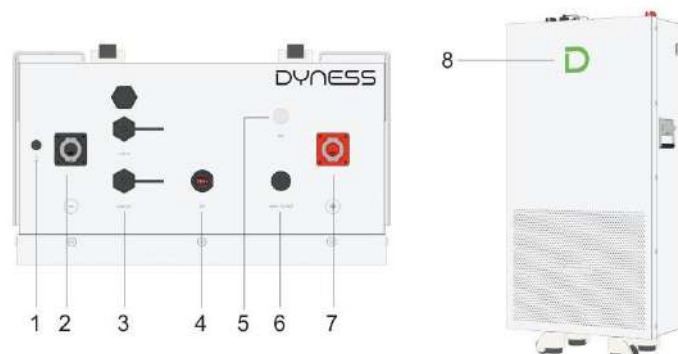
Figure 2-1 PowerBrick Pro the Sketch of Front Interface
